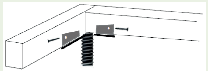
40mm Screws Through Plinth Brackets
